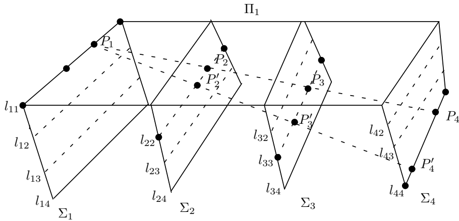
FIGURE 1. Constructing a new plane (the 16 dots).
