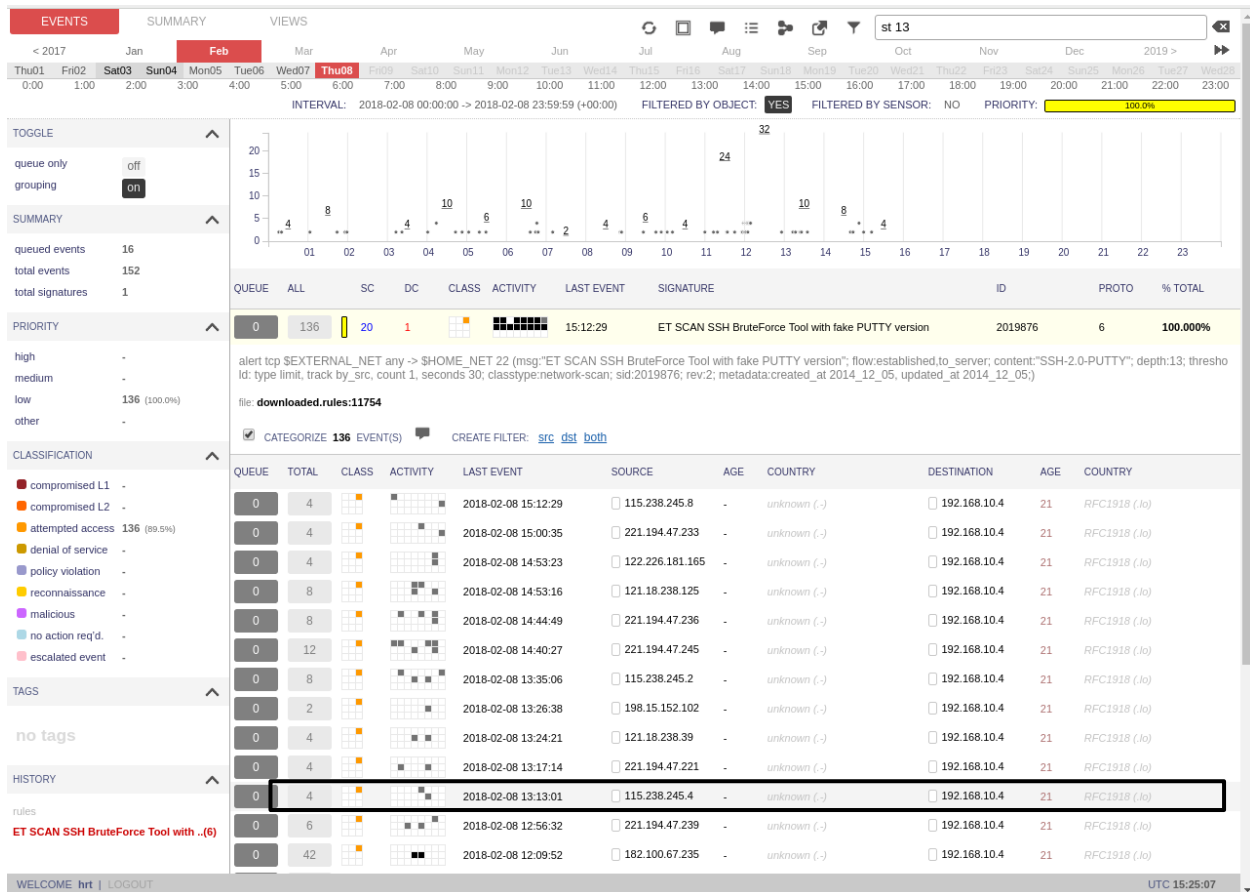
Figure3: Squert tools
